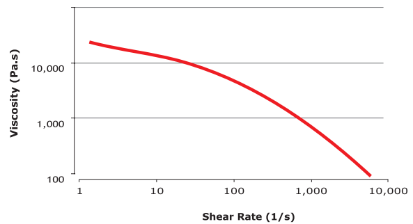
Shear-Viscosity @ 190 °C
